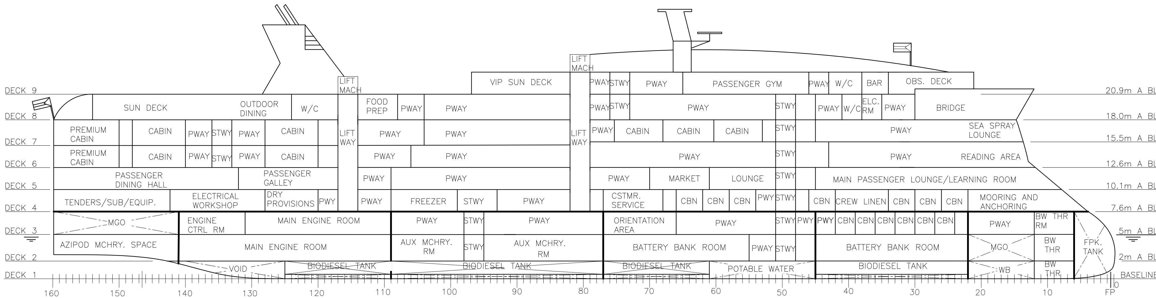
INBOARD PROFILE
