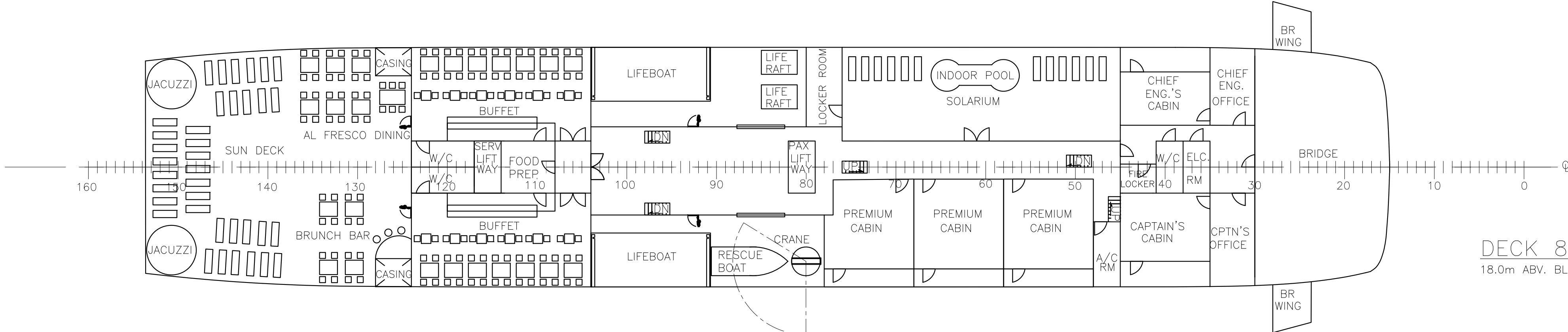
DECK 9 20.9m ABV. BL
