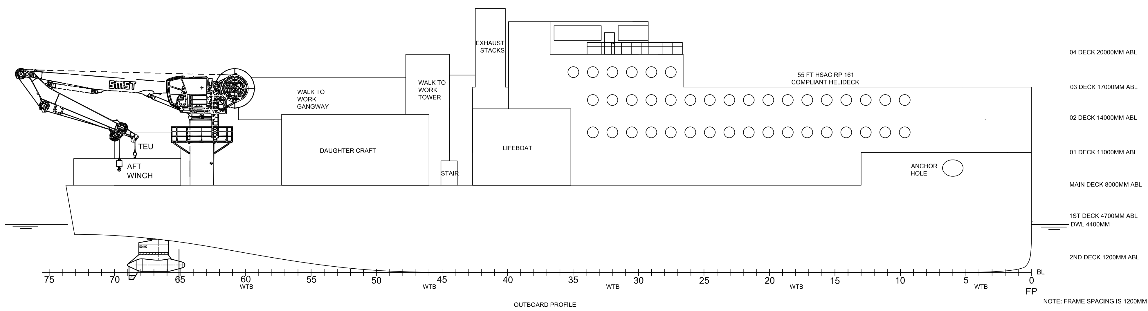
OUTBOARD PROFILE
