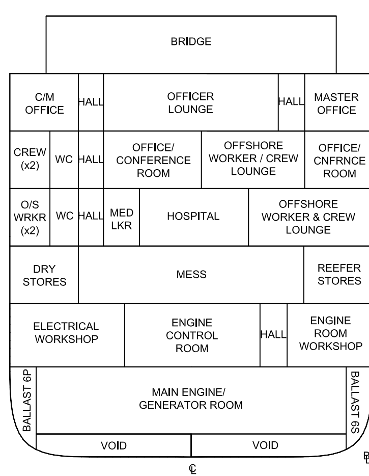
MIDSHIP ARRANGEMENT
