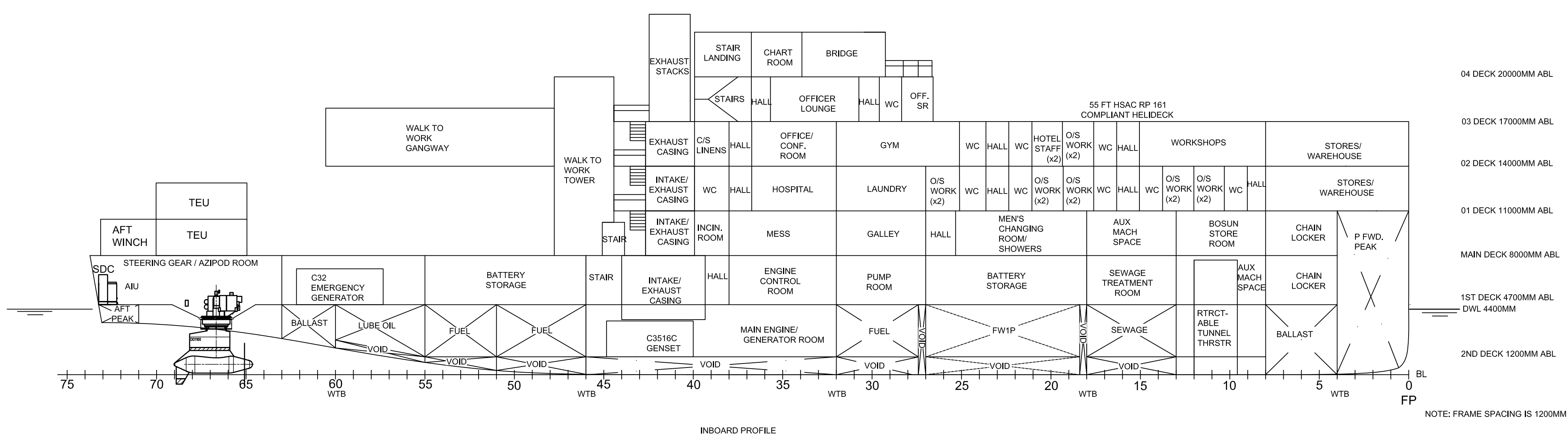
INBOARD PROFILE
