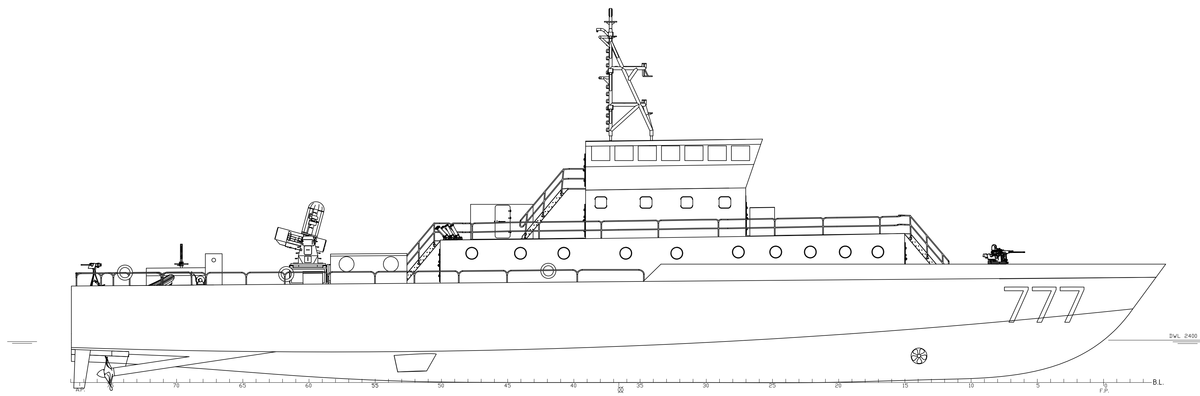
OUTBOARD PROFILE
