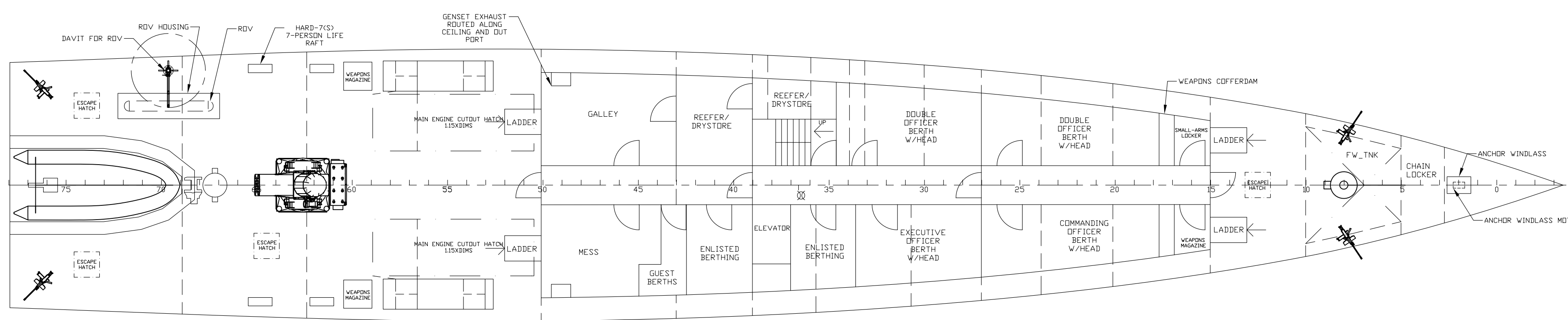
MAIN DECK (5723 mm ABL)
