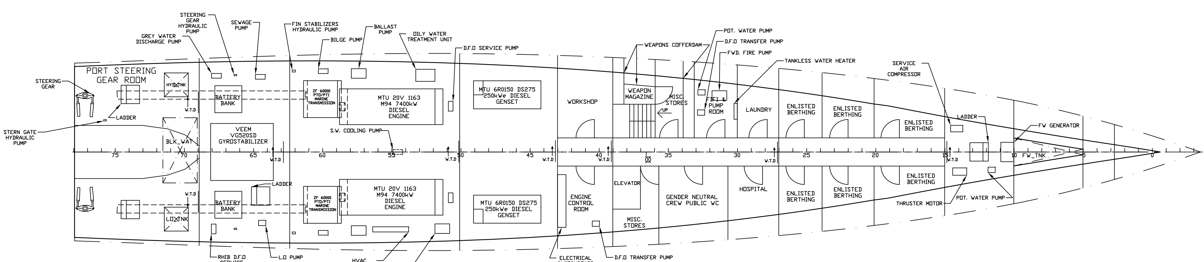
SECOND DECK (2766 mm ABL)
