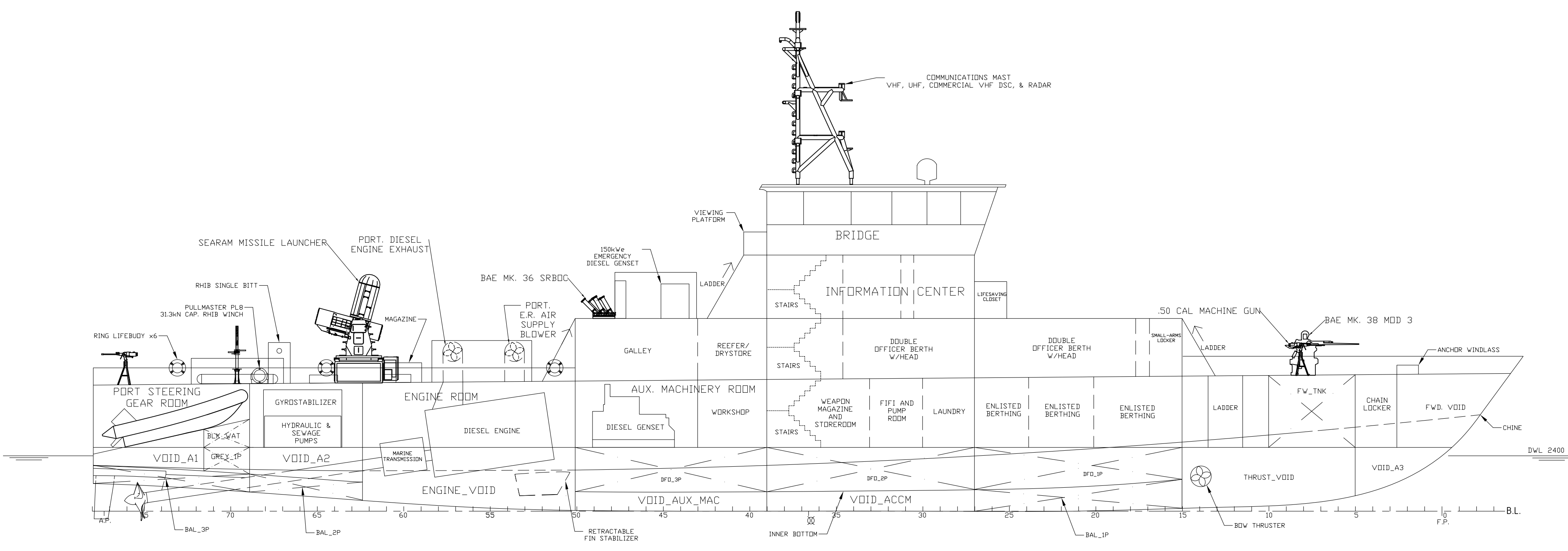
INBOARD PROFILE
