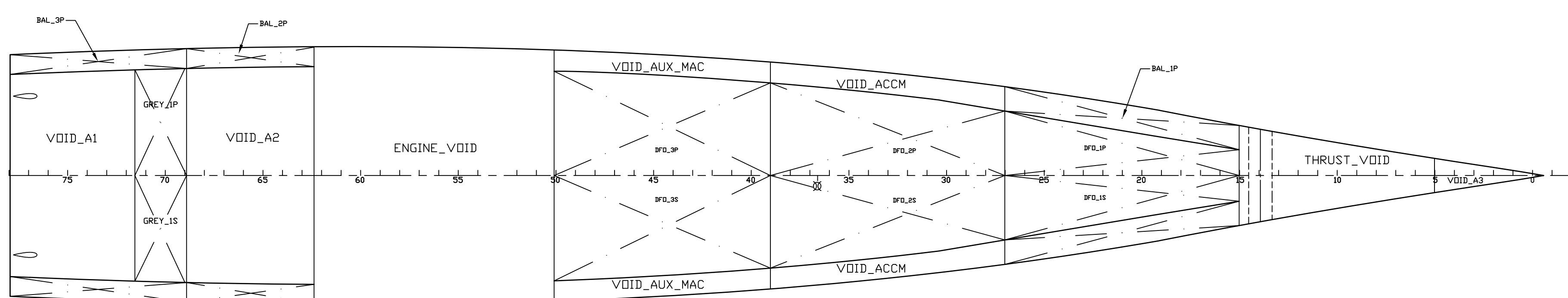
TANK TOP (2766 mm ABL)
