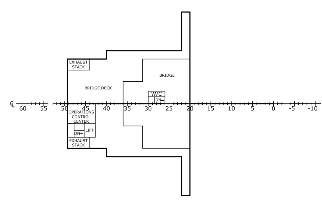
PILOTHOUSE DECK (36m ABL)
