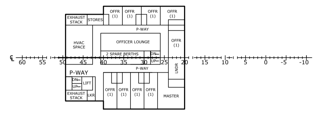
SUPER 3 (33m ABL) OFFICER DECKHOUSE
