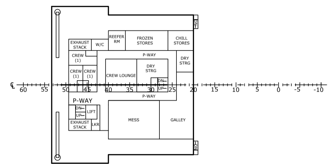
SUPER 2 (30m ABL)
