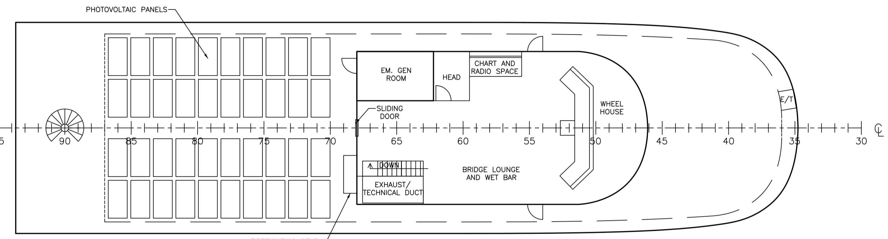
THIRD DECK
