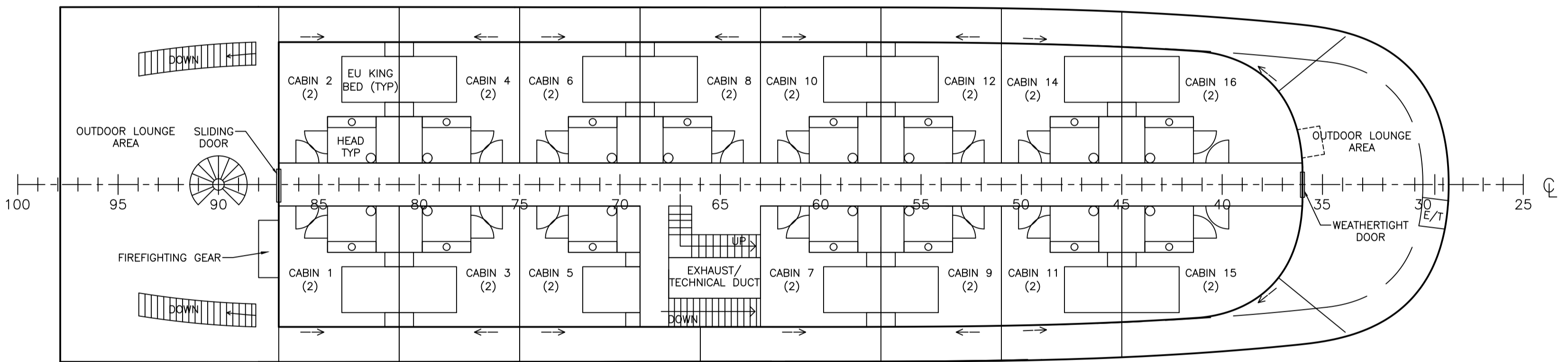
SECOND DECK
