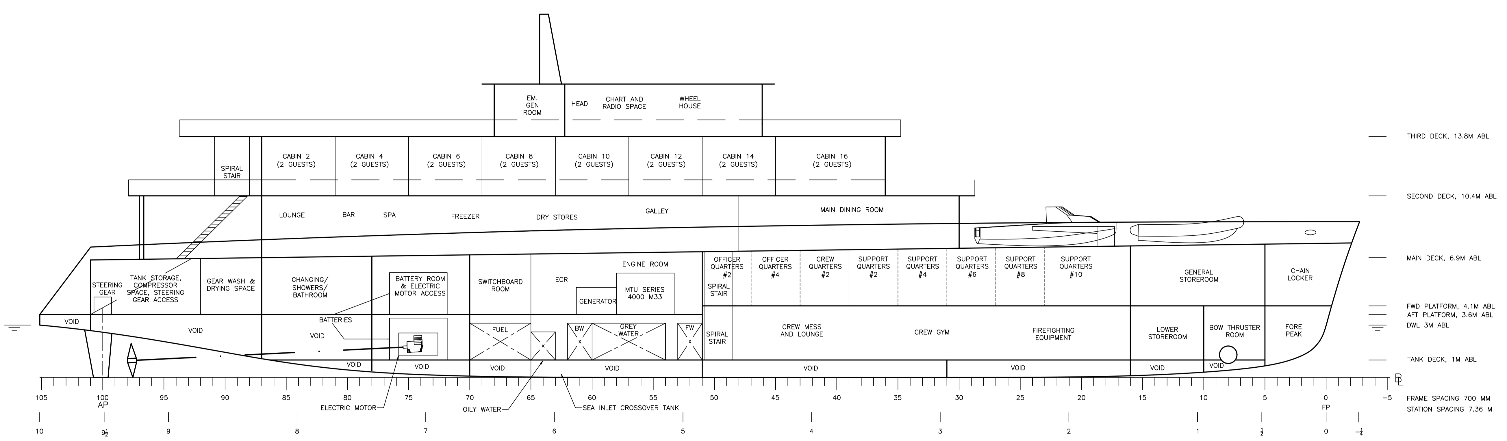
INBOARD PROFILE
