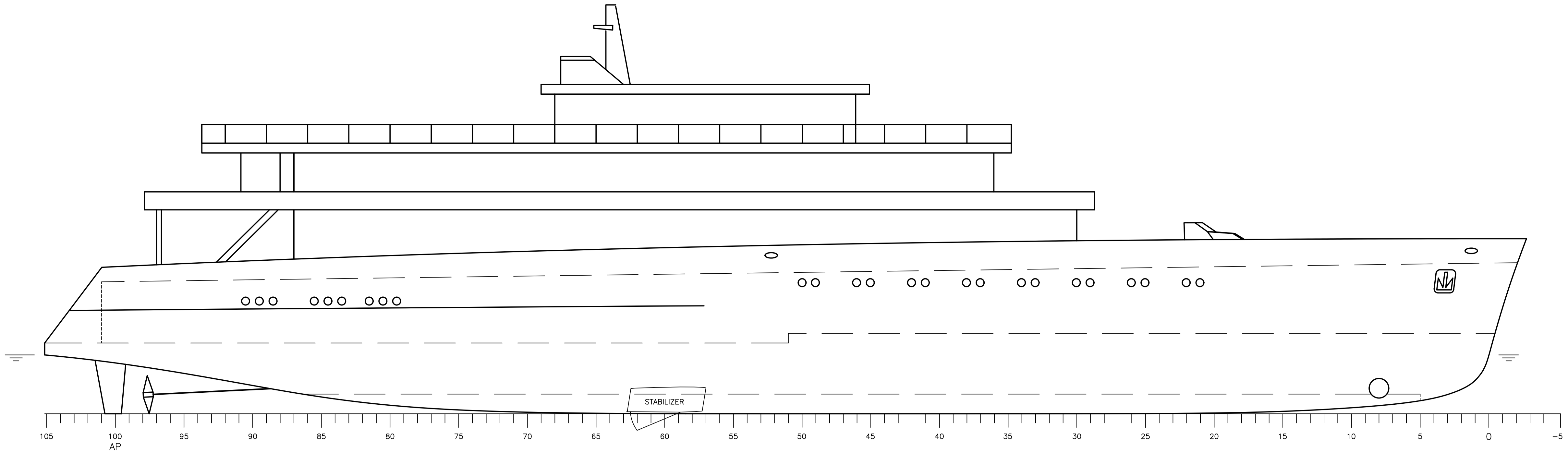
OUTBOARD PROFILE
