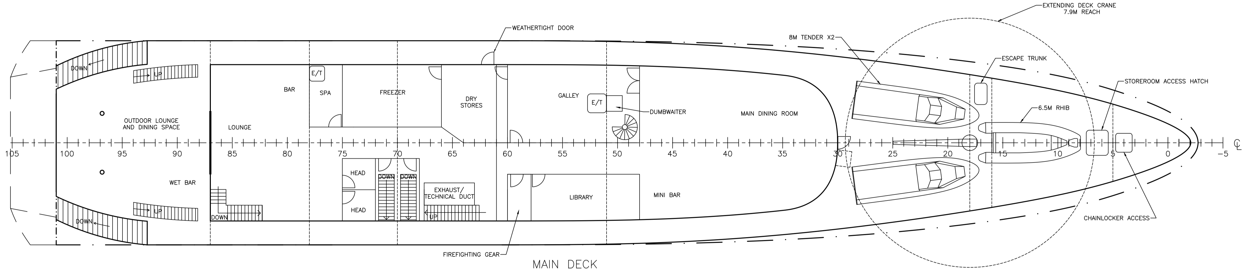
MAIN DECK
